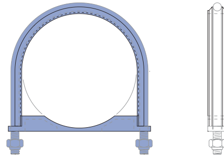
8" thru 12" assembly.
